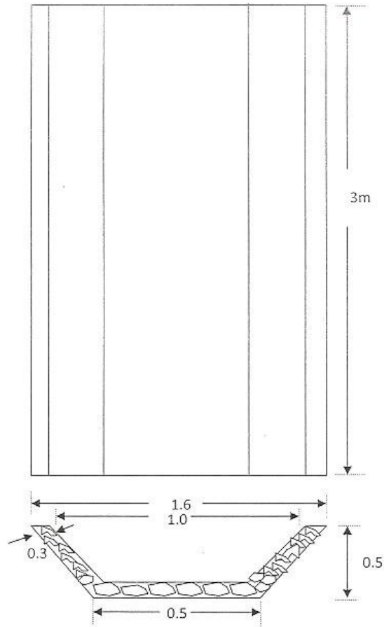
Fig. cross sectional and top view of the channel before silt trap
