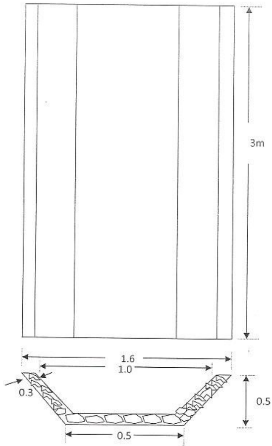
Fig. cross sectional and top view of the out let channel
