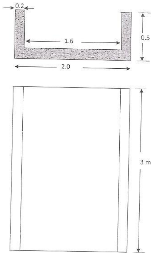
Fig. cross sectional and top view of the approach channel of the inlet
