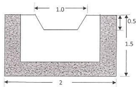
X-X cross sectional view
